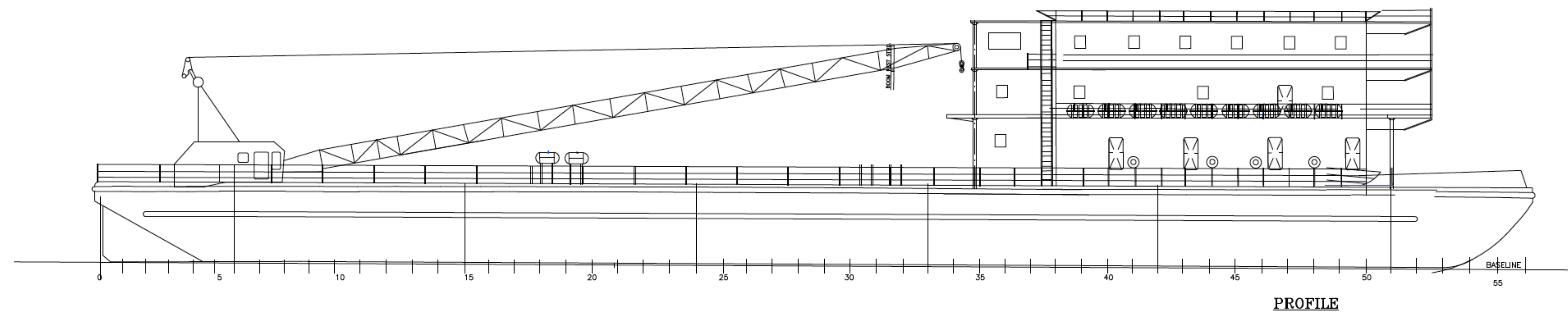
PROFILE
