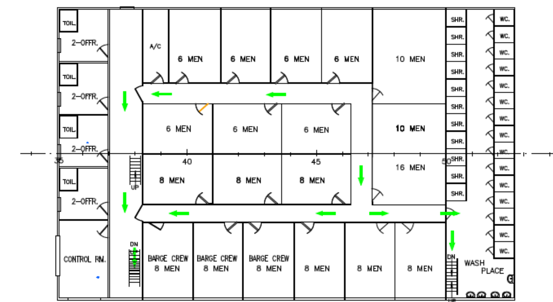
02 DECK
