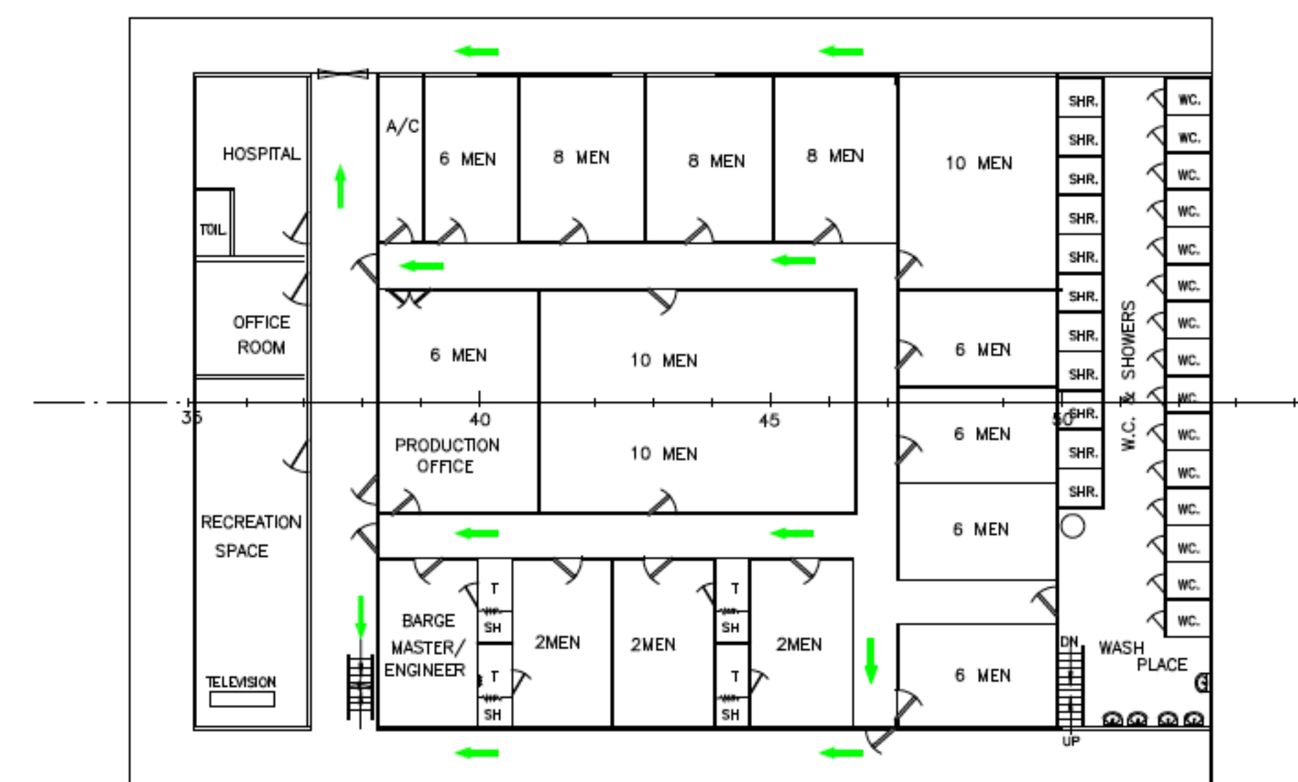
01 DECK
